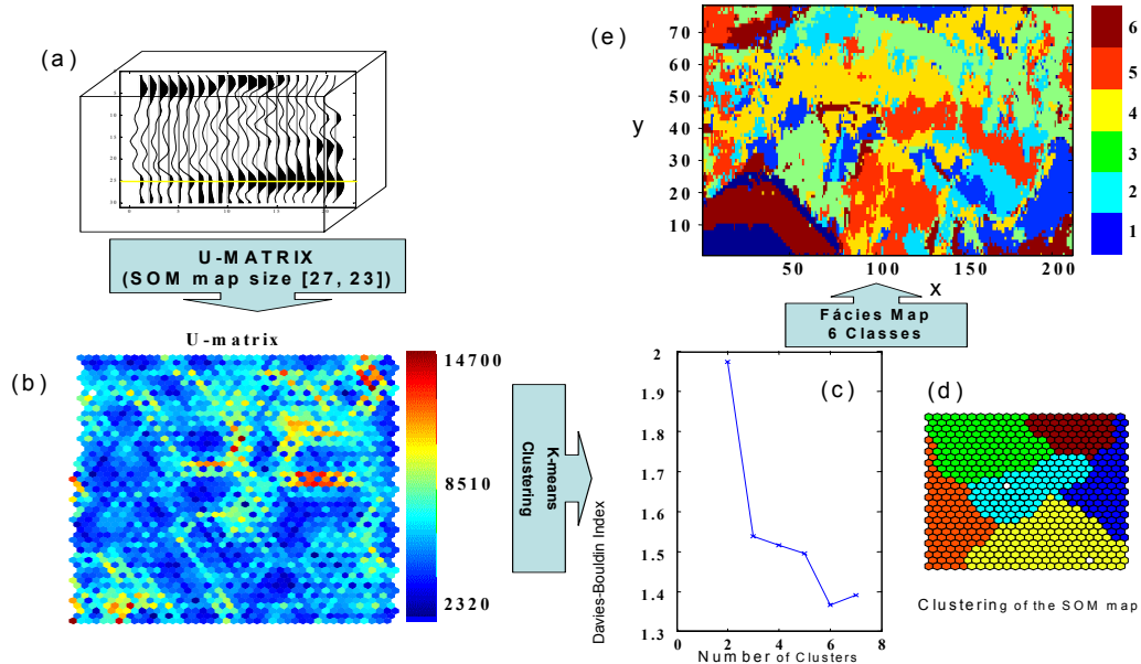
Figure 2: Facies analysis methodology. This example uses 32 seismic amplitudes around the reservoir bottom as input attribute. (a) seismic amplitudes; (b) The U-matrix of a 27x23 SOM map; (c) Davies-Bouldin index with 6 class minima; (d) clustering of SOM map and (e) facies map
