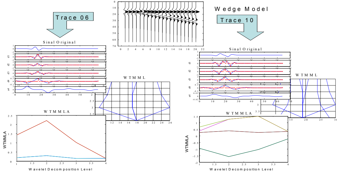
Figure 1: Synthetic signals; its wavelet à trous decomposition; WTMML and WTMMLA.
